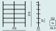
8916 14 shelves - 4 struts
