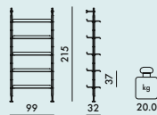
8915 10 shelves - 3 struts
