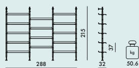
8916 14 shelves - 4 struts
