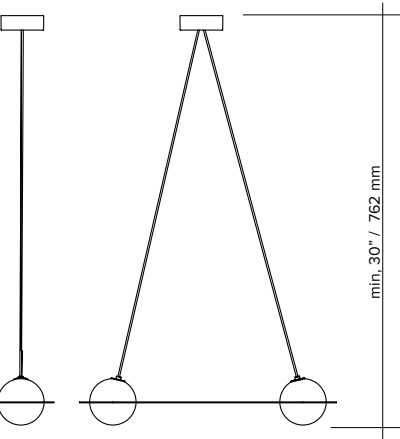
angled wires
