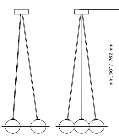
angled wires
