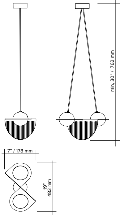
angled wires
