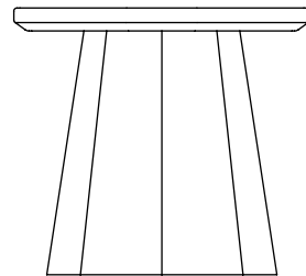
Pine Table small H: 40,6 x Ø45 cm
