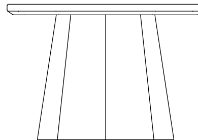
Pine Table large H: 44,6 x Ø65 cm
