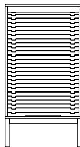
Jalousi Cabinet low H: 101,5 x L: 55 x D: 40 cm
